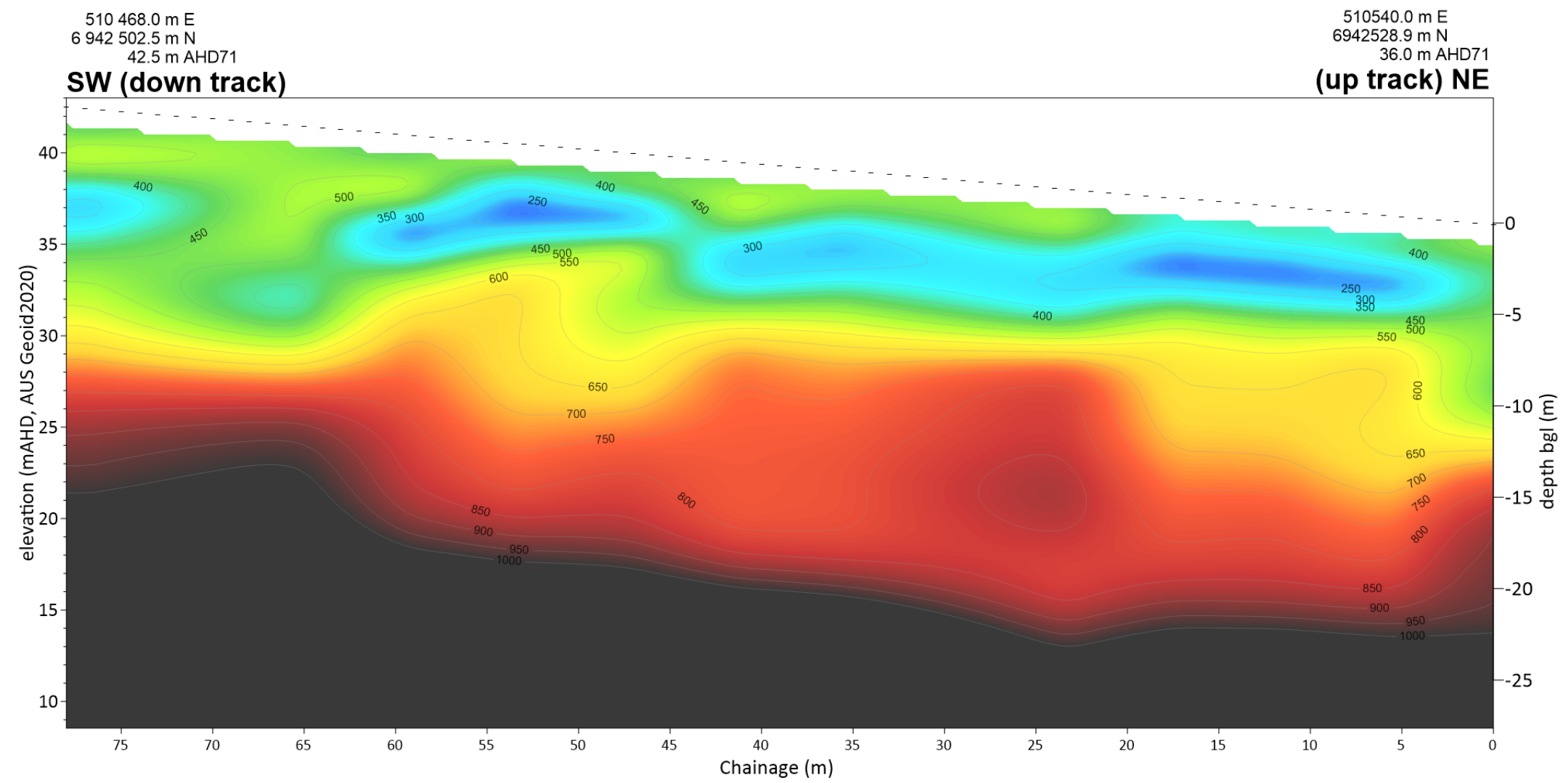
Seismic Line MASW AU-GP 137
